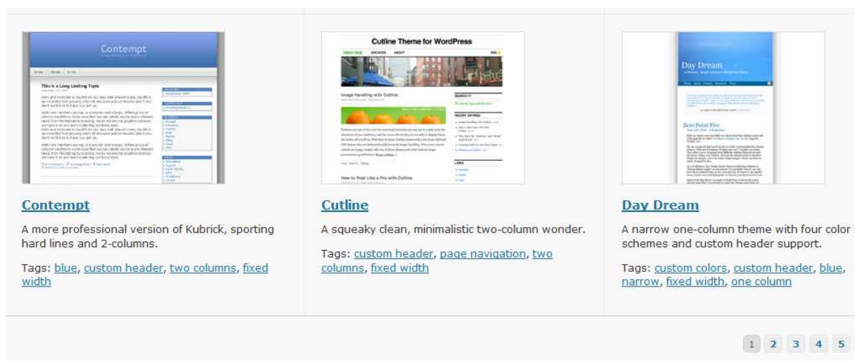
Gambar 15. Aneka themes
