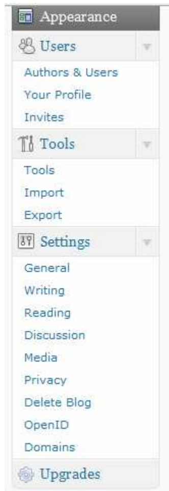
Gambar 20. Submenu Setting
