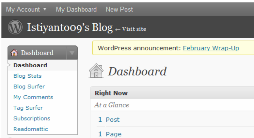
Gambar 9. Dashboard wordpress
